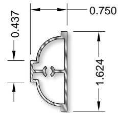
Profile 990301
