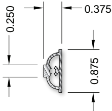
Profile 990300
