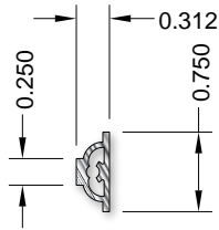
Profile 990394/990392
