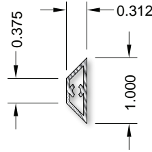
Trapezoidal 990882
