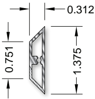
Trapezoidal 990880
