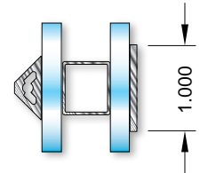
Triple With Trap 1" IG Unit
