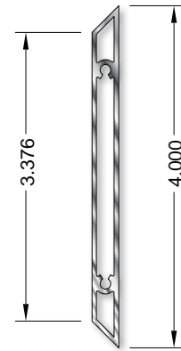
Trapezoidal 990333
