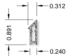
Frame Filler 990388 (Use Only With 990315 Or 990871 Grid)
