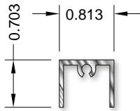
Frame Filler 990343
