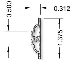
Profile 990393/990391
