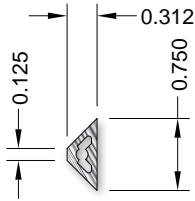
Trapezoidal 990304/990315
