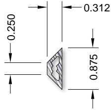
Trapezoidal 990326
