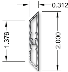
Trapezoidal 990306
