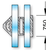
Triple With Trap 5/8" IG Unit
