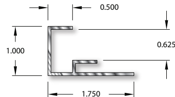
5/8" Drywall Trim (No Clip) 999440
