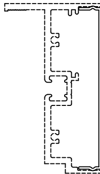
Caulk Stop 3 1/2" Products 956801
