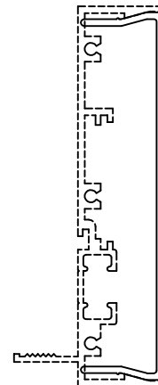
Caulk Stop 4 1/2" Products 951501
