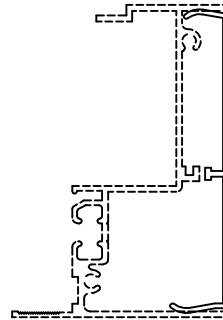
Caulk Stop 3 1/4" Products 952001
