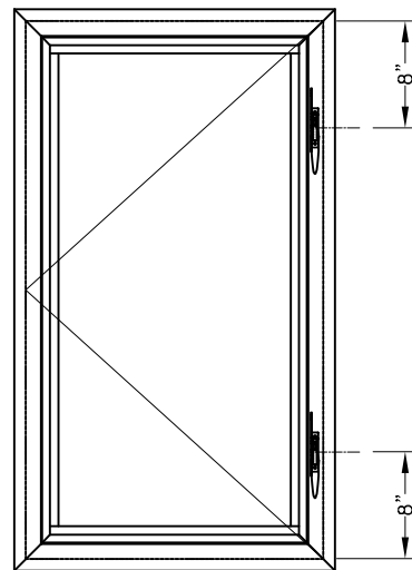
ELEVATION Outswing Casement Window (Viewed From Inside) Vent Heights From 25" To 58" 8" From Each End Of Vent
