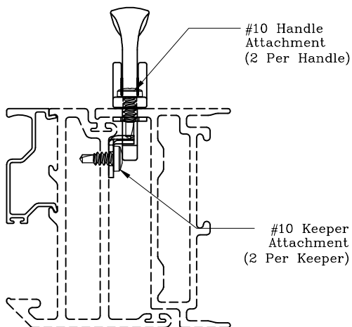
Single Point Lock Handle and Keeper Attachment
