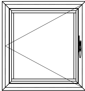
ELEVATION Outswing Casement Window (Viewed From Inside) Vent Heights Up To 24" (1) Lock At Midpoint Of Vent
