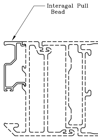
Pull Handle Attachment
