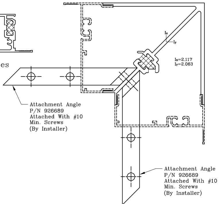
90° Corner Mullion
