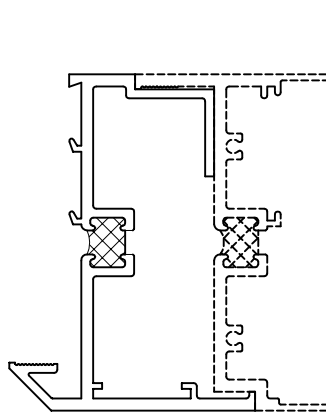
Outswing Fixed Sightline Adapter
