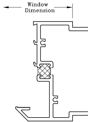
Male Slip Mullion Fixed Jamb
