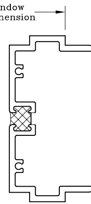
Universal Male Slip Mullion
