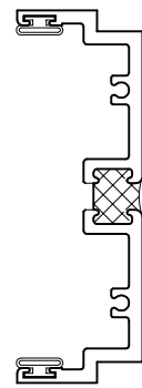
Universal Female Slip Mullion
