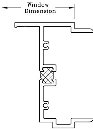
Male Slip Mullion Inswing/Outswing Jamb
