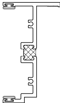
Female Slip Mullion Inswing/Outswing Jamb
