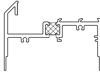
Fixed Head, Jamb, and Sill
