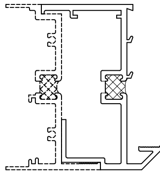
Inswing Fixed Sightline Adapter
