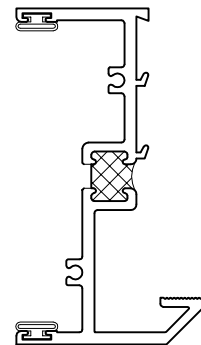
Female Slip Mullion Fixed Jamb
