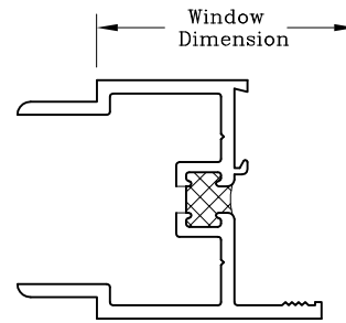
Male Slip Mullion Fixed Jamb
