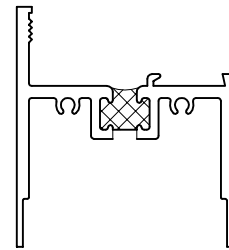
Fixed Frame
