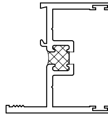
Female Slip Mullion Fixed Jamb
