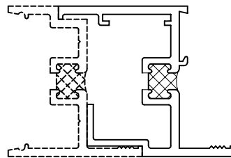
Inswing Fixed Sightline Adapter
