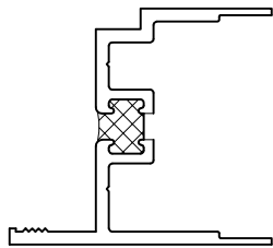
Inswing/Outswing Jamb
