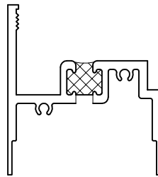
Inswing Head Sill
