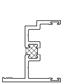
Female Slip Mullion Inswing/Outswing Jamb
