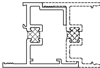
Outswing Fixed Sightline Adapter
