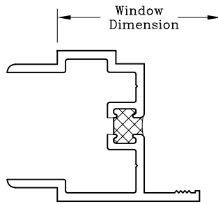
Male Slip Mullion Inswing/Outswing Jamb
