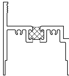
Outswing Head/Sill
