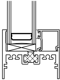
1" IG Glazing Bead
