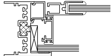
Lift-In Guardian Vertical Glazing Bead
