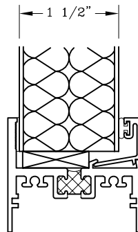
1 1/2" Panel Glazing Bead
