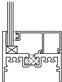
Single Glaze (1/8", 3/16", 1/4") Glazing Bead
