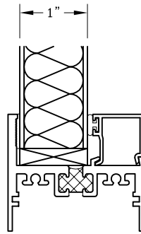
1" Panel Glazing Bead
