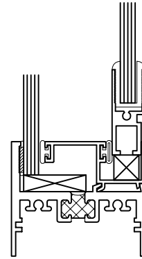
Lift-In Guardian Horizontal Glazing Bead
