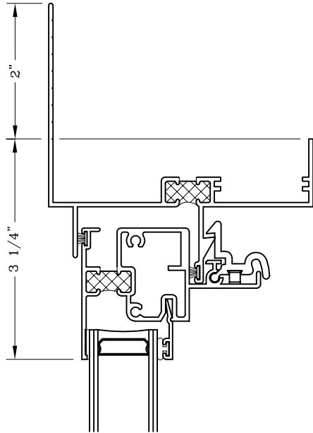
2" Flange Frame (Head Shown)
