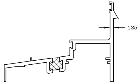
Single Hung Equal Leg Sill w/Snap Barb
