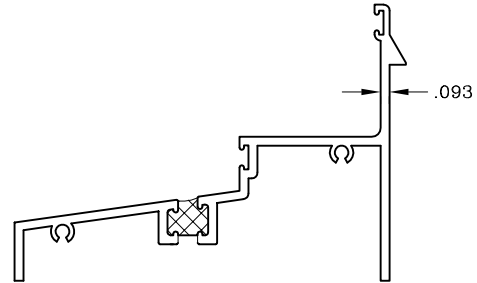
Double Hung Equal Leg Sill w/Snap Barb
