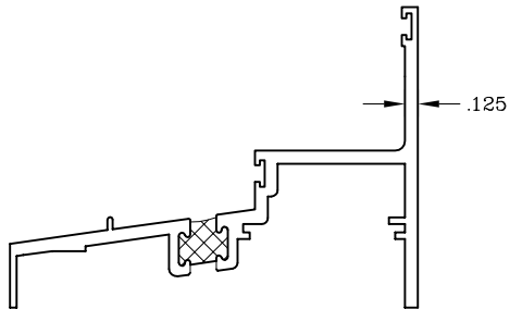
Single Hung Equal Leg Sill
