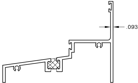
Double Hung Equal Leg Sill
