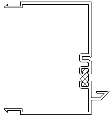
.062 Wall Extended Leg Male Jamb
