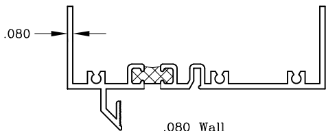
.080 Wall Head
