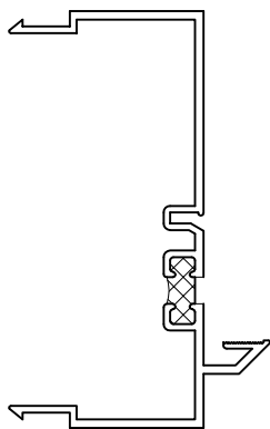
.080 Wall Self-Mull Jamb
