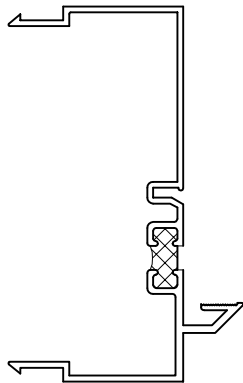
.062 Wall Self-Mull Jamb
