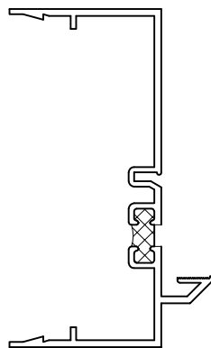
.080 Wall Extended Leg Jamb
