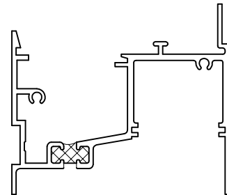
AW Sill Equal Leg
