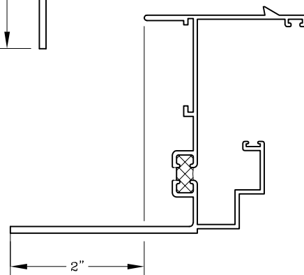
Operating Vent Flange Frame
