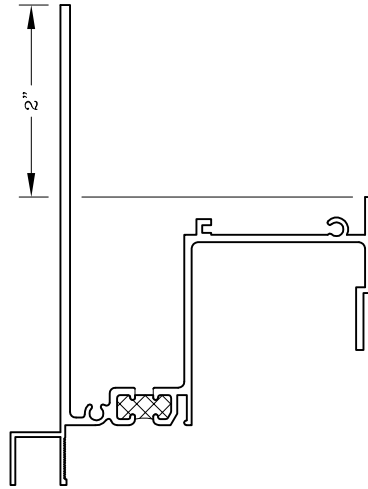
Flange Leg Head w/ Screen
