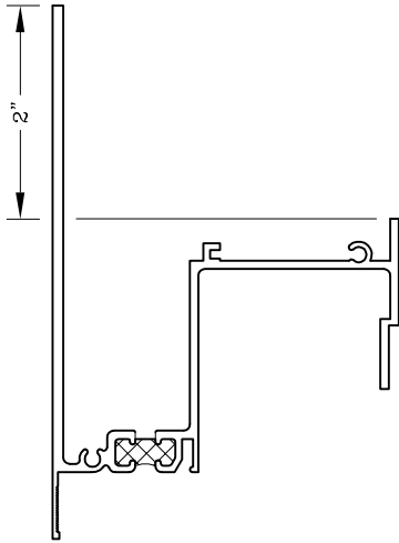
Flange Leg Head w/o Screen
