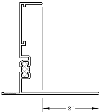
Non Operating Vent Flange Frame
