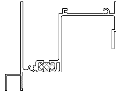
Equal Leg Head w/ Screen
